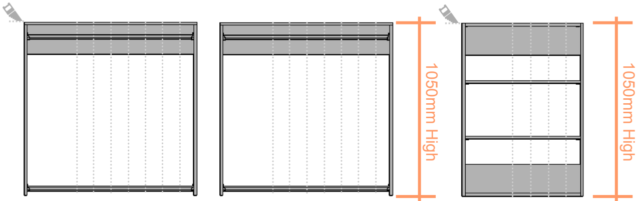
Shelves with 2 Clothes Rails 300 to 1000 wide - 295 to 395 deep
